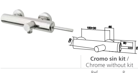
Monomando ducha / Single lever shower mixer
